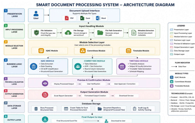
Fig 3.1. Architecture Diagram of the Smart Document Processing System.
